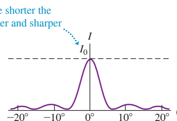
Figure 36.10 The single-slit diffraction pattern depends on the ratio of the slit width a to the wavelength \lambda .
